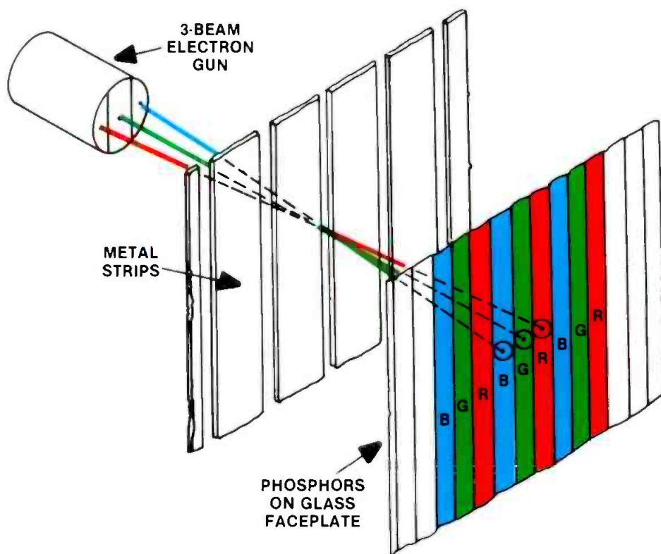
Figure 5. A single-gun CRT has a flat faceplate and produces the fewest convergence problems because all three beams are handled by a single electronic lens. The picture is bright, but signal degradation may be less visible than with a dot-type CRT.
