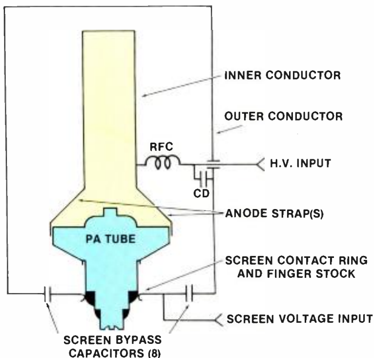
Figure 5. The 1/2-wavelength PA cavity in its basic form.
