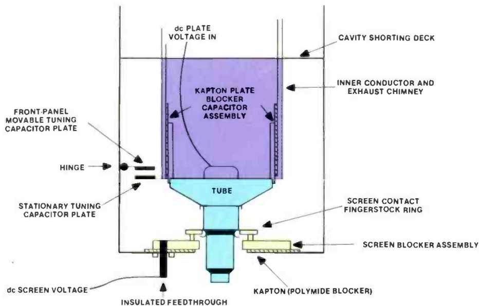
Figure 1. The layout of a common type of \frac{1}{4} -wavelength PA cavity.
