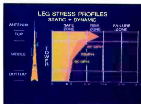
Figure 3. The differences in the static and dynamic leg stress on the same towers as in Figure 2, based on different static design wind speeds.
