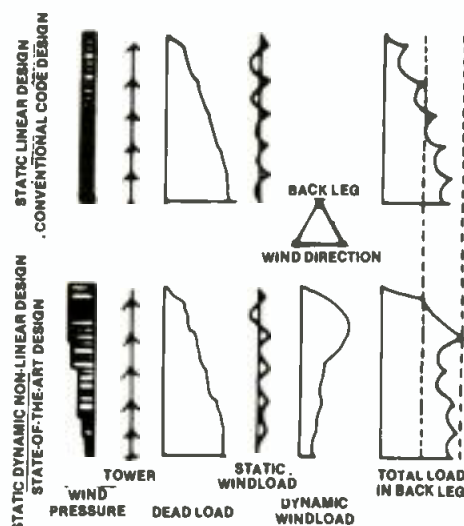
Figure 4. When dynamic forces are considered, some guyed towers may be at more of a risk than owners may realize.
