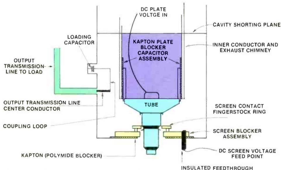
Figure 14. The position of the inductive coupling loop in a \frac{1}{4} -wavelength FM cavity amplifier. Note that the loop is located away from the points of maximum RF voltage and current.
