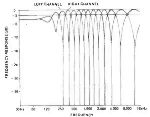
Figure 3. Stereo synthesis begins by filtering the audio into either narrowband or wideband signals. These signals are then combined to create an L-R signal, which is used to generate the discrete left and right stereo signals.
