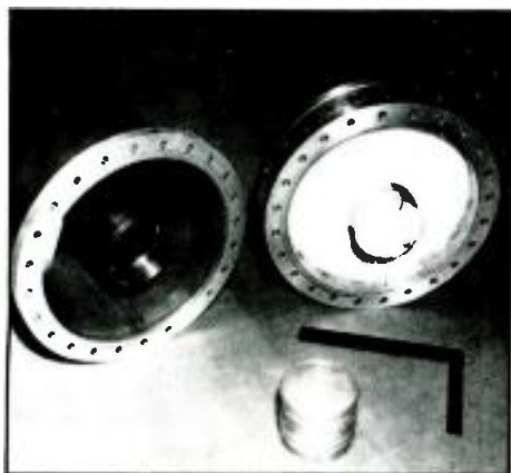
The world's largest known coax. 14 inches in diameter, was designed for a cyclotron.
