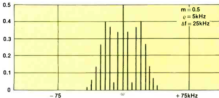
Figure 2. RF spectrum with a modulation index of 5.
