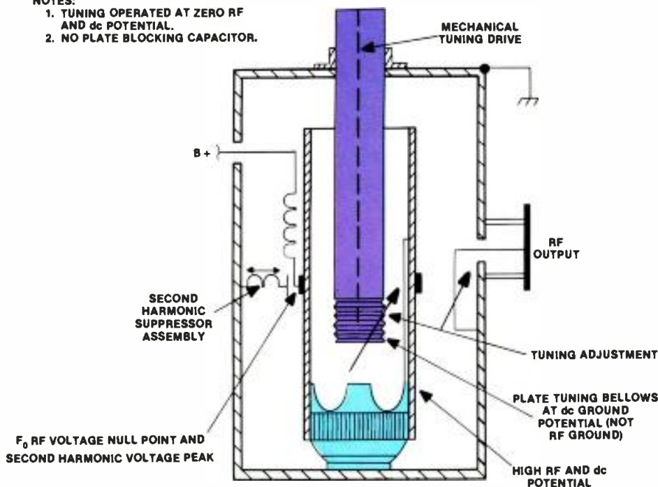
Figure 9. The basic design of a folded \frac{1}{2} -wavelength cavity.
