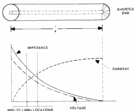
Figure 3. A graph of the RF current (...), RF voltage (—) and RF impedance (—) for a 1/4-wavelength shorted transmission line. At the feed point RF current is zero, RF voltage is maximum and RF impedance is infinite.
