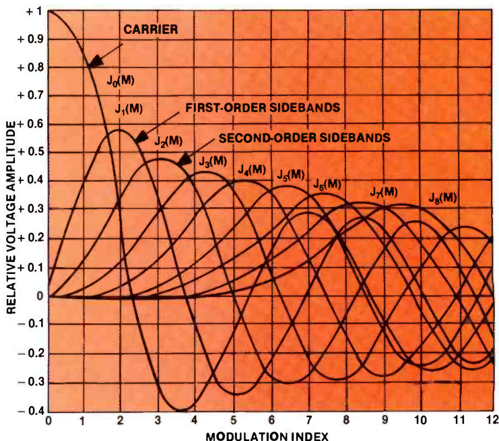
Figure 4. The Bessel function graph illustrates the relationship between the carrier and side-band amplitudes to modulation index.
